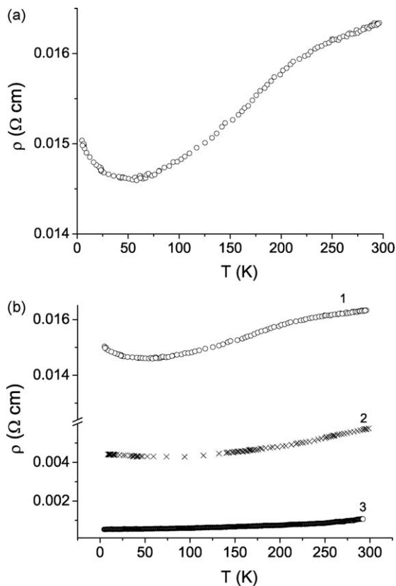
Fig. 3. (a) Temperature dependence of the electrical resistivity of MDF-SiC/Si composite (with 30 vol.% of Si). (b) Comparison of temperature dependences of the electrical resistivity of MDF-SiC/Si composite (curve 1) with 30 vol.% of Si and of the bio-SiC derived from eucalyptus (curve 2 from Ref. 21 ) and from beech (curve 3 from Ref. 22 ).
