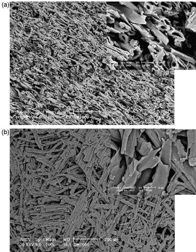
Fig. 1. SEM micrographs of MDF-C taken perpendicular (a) and parallel (b) to the direction of compacting the parent MDF boards.
