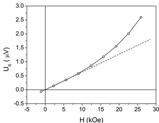
Fig. 5. Dependence of the Hall voltage U_R at 77 K on the magnetic field H for MDF-SiC. Dashed line corresponds the linear dependence U_R(H) .
