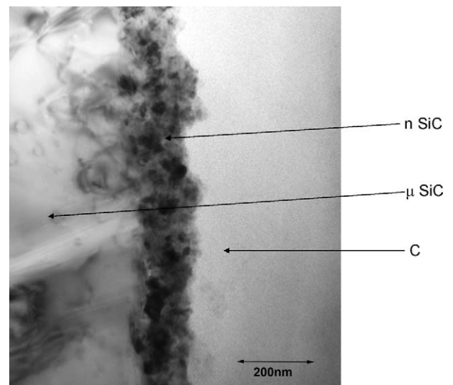
Fig. 6. Electron microscope image of the MDF-SiC demonstrating the presence of micro- and nanocrystalline SiC and residual amorphous carbon.
