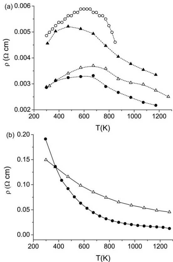
Fig. 7. (a) Temperature dependences of the electrical resistivity for MDF-SiC/Si composite derived from MDF boards with the density in the 0.6–0.8 g/cm 3 limits and Si content in the 20–50 vol.% range. (b) Temperature dependences of the electrical resistivity of two MDF-SiC samples which were obtained on the base of the same MDF board (the density 0.8 g/cm 3 ), but their MDF-precursors were cut from its different regions.
