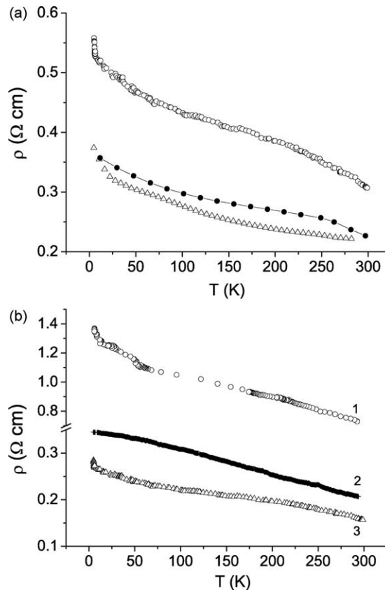
Fig. 4. (a) Temperature dependences of the electrical resistivity of MDF-SiC samples which were obtained on the base of the same MDF board, but their MDF-precursors were cut from its different parts. (b) Temperature dependences of the electrical resistivity of bio-SiC samples derived from eucalyptus (1), beech (2) and MDF board (3), which are plotted with correction for the samples porosity.
