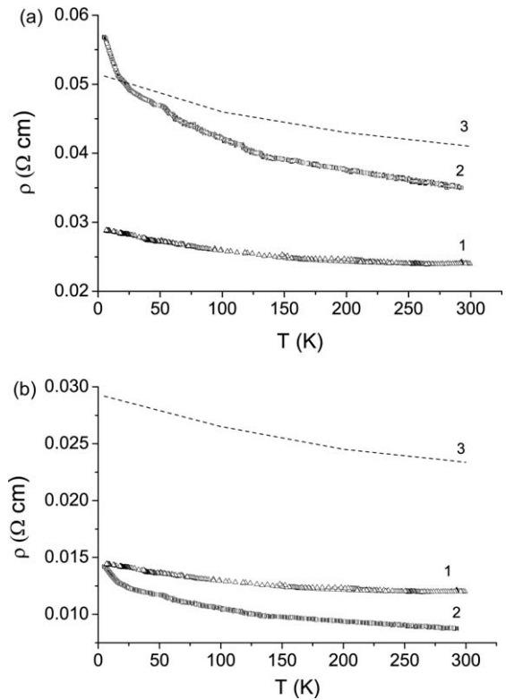
Fig. 2. Temperature dependences of resistivity of porous biocarbon derived from MDF board (1), white pine (curve 2 from Ref. 31 ) and eucalyptus (curve 3 from Ref. 30 ) woods without (a) and with (b) correction for the porosity.
